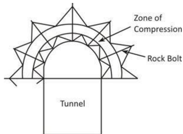
Formation of a strengthened zone through rock bolt
