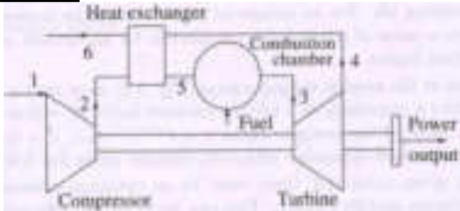
Fig. 45. Simple gas turbine with heat exchanger
