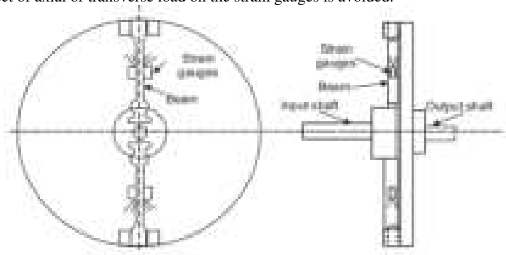
Fig. 33. Transmission dynamometer
