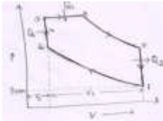
Fig. 9. Dual cycle
