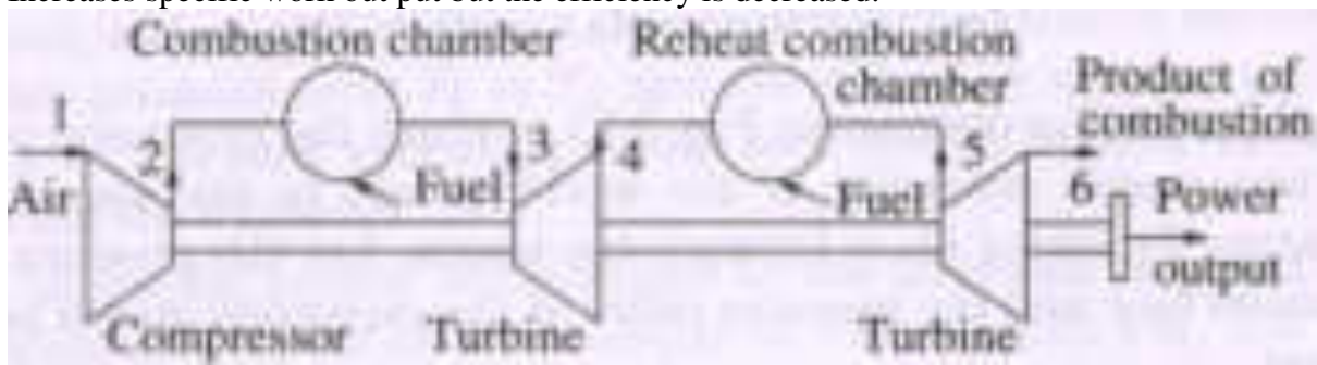
Fig. 46. Arrangement of reheat cycle
