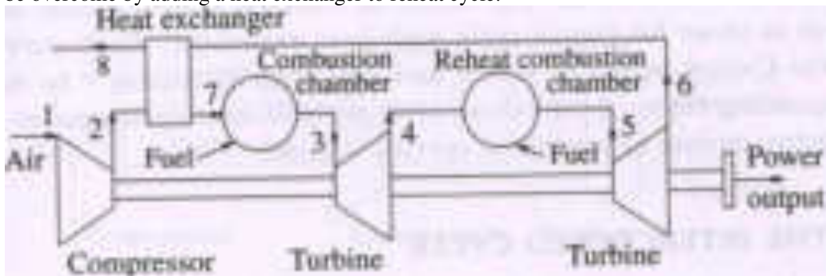
Fig. 47. Arrangement of reheat cycle with heat exchanger
