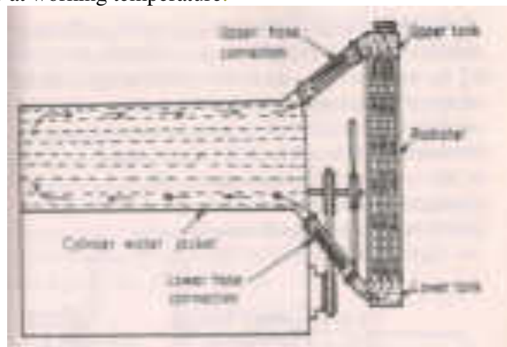
Fig. 37. Thermo-syphon cooling
