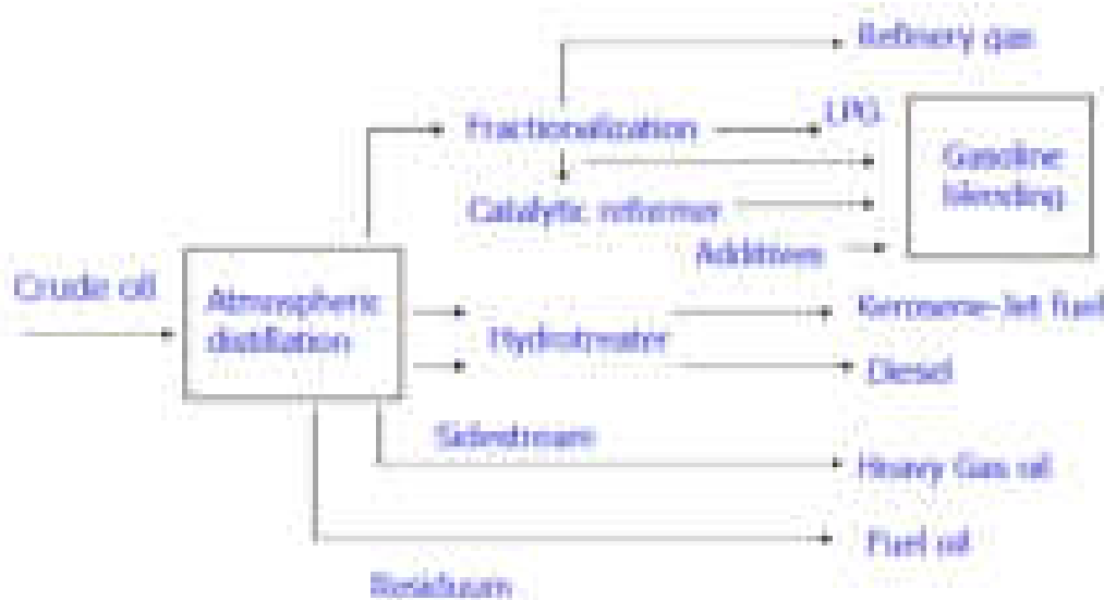
Fig. 10. Refinery processes
