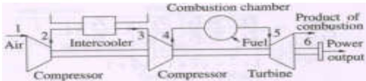
Fig. 48. Arrangement of intercooled cycle
