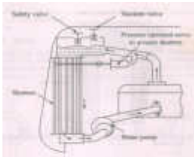
Fig. 39. Pressurised system
